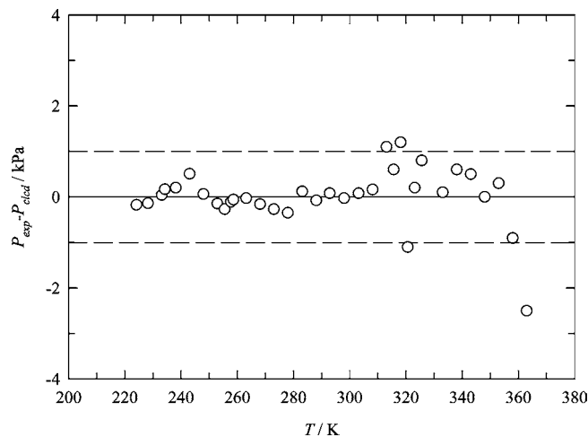
Figure 4. Scatter diagram of the saturated pressure—absolute deviations between experimental pressures ( P_{\text{exp}} ) and pressures calculated from REFPROP 8.0 ( P_{\text{calc}} ).
