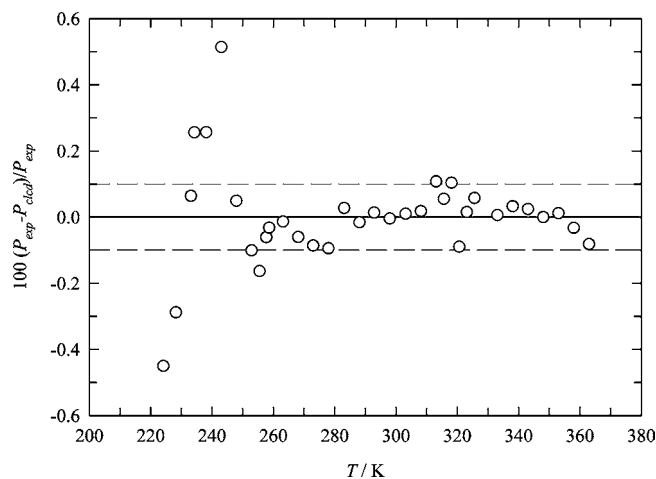
Figure 5. Scatter diagram of the saturated pressure—relative deviations between experimental pressures ( P_{\text{exp}} ) and pressures calculated from REFPROP 8.0 ( P_{\text{calc}} ).
