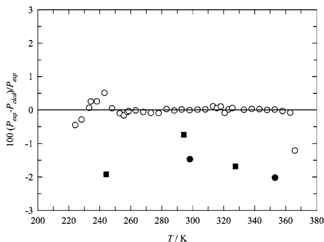
Figure 6. Scatter diagram of the saturated pressure—relative deviations between experimental pressures ( P_{\text{exp}} ) and pressures calculated from REFPROP 8.0 ( P_{\text{calc}} ): ●, ref 7; ■, ref 14.
