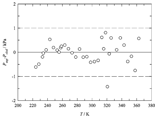
Figure 2. Scatter diagram of the saturated pressure—absolute deviations between experimental pressures ( P_{\text{exp}} ) and pressures calculated from the fit with the Wagner equation, eq 1 ( P_{\text{calc}} ).
