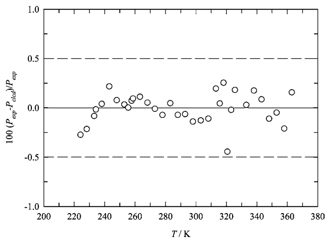
Figure 3. Scatter diagram of the saturated pressure—relative deviations between experimental pressures ( P_{\text{exp}} ) and pressures calculated from the fit with the Wagner equation, eq 1 ( P_{\text{calc}} ).
